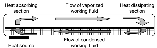
Figure 2 Circulation of working fluid in pera-flex.
